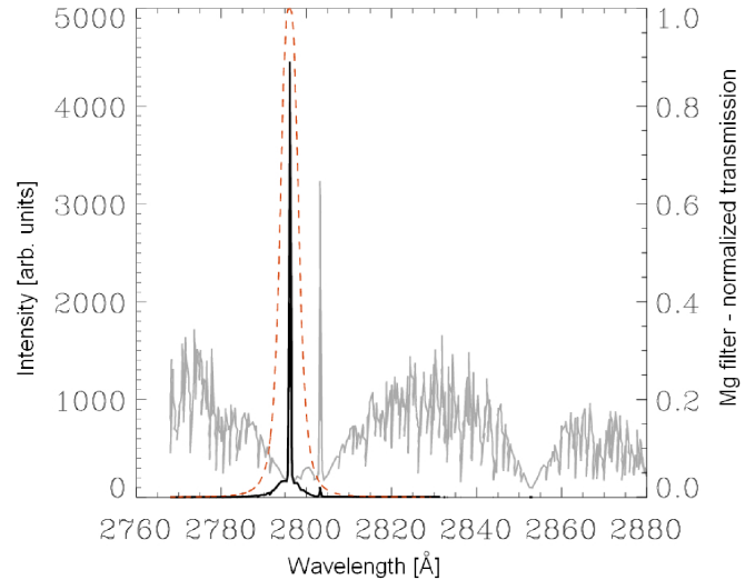
FIG. 1.— Observed Mg II h&k spectrum in plage (solid grey) and the same multiplied by the SuFI filter transmission curve (solid black; multiplied by 10 for better display). The SuFI Mg filter transmission profile is overplotted with corresponding y axis on the right (dashed red).
